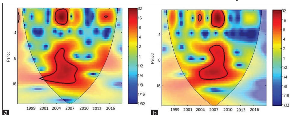
Figure 3: Continuous wavelet power spectra of ENG and CO 2
