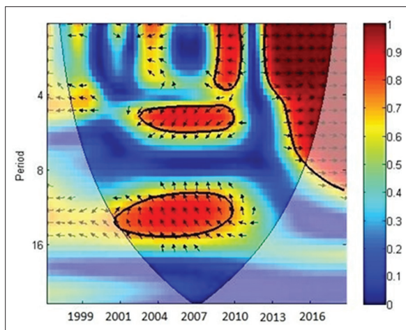
Figure 2: (a-b) Wavelet coherence power spectra of RENW-CO 2
