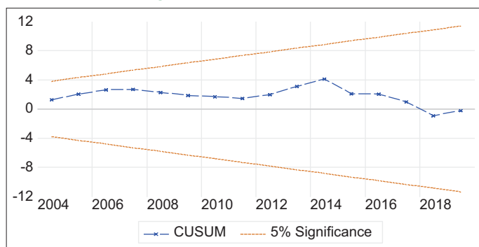
Figure 2: Plot of CUSUM test
