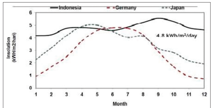
Figure 1: Radiation Distribution Graph in Indonesia (Widayana, 2012).
